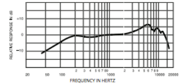
Frequency Response
