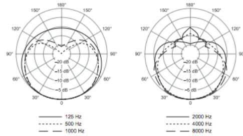
Polar Pattern
